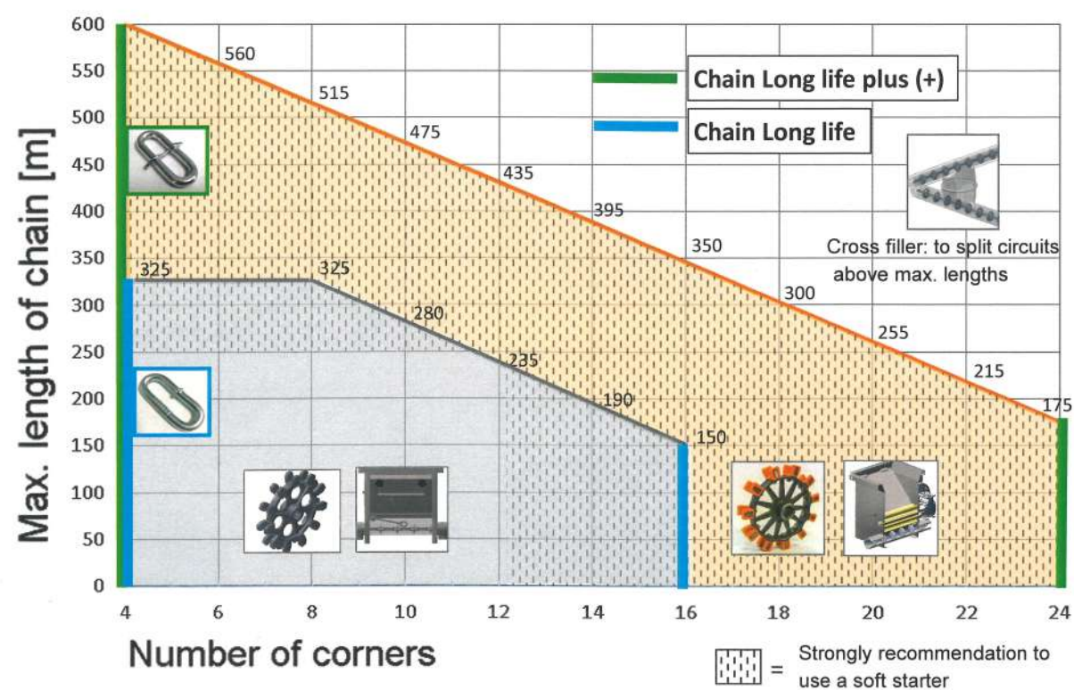
Dimensioning diagram for Chainfeed 60 mm
