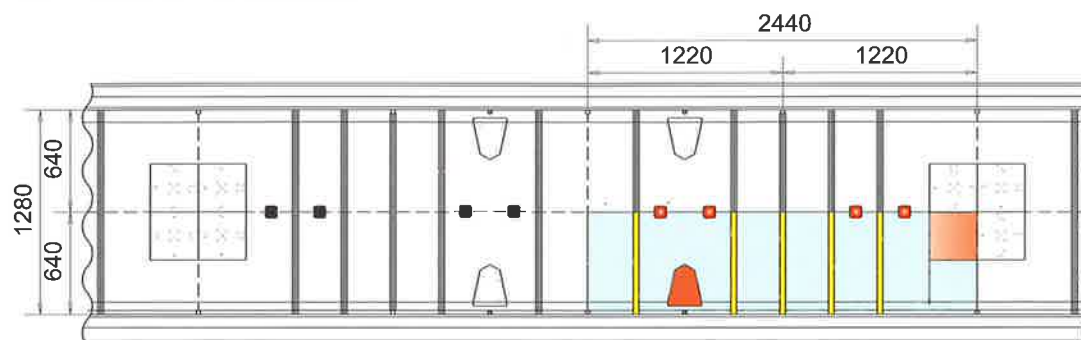
Box 2440 x 640 - 20 capi/birds
